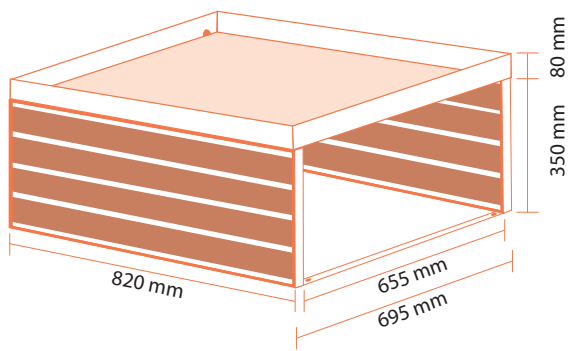
Lawn mower garage Bloom | Art. No. 1101
