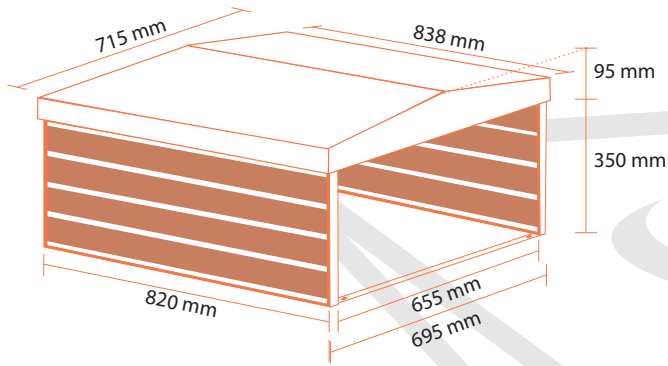
Lawn mower garage Lodge | Art. No. 1100
